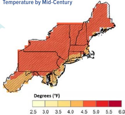
Projected Increase in Annual Temperature by Mid-Century
