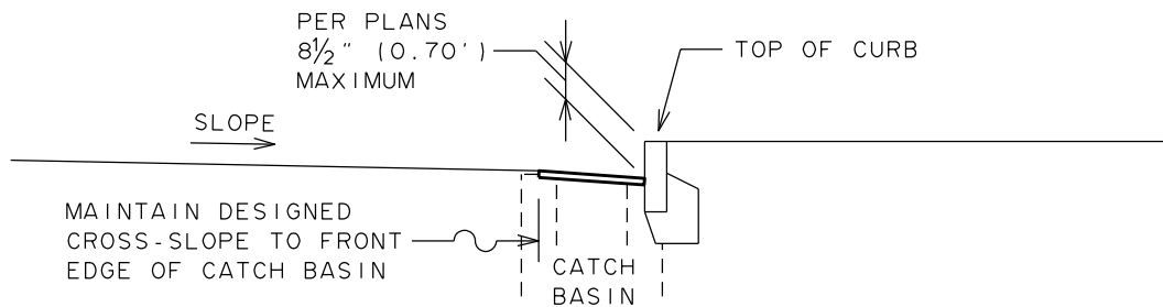
SECTION
