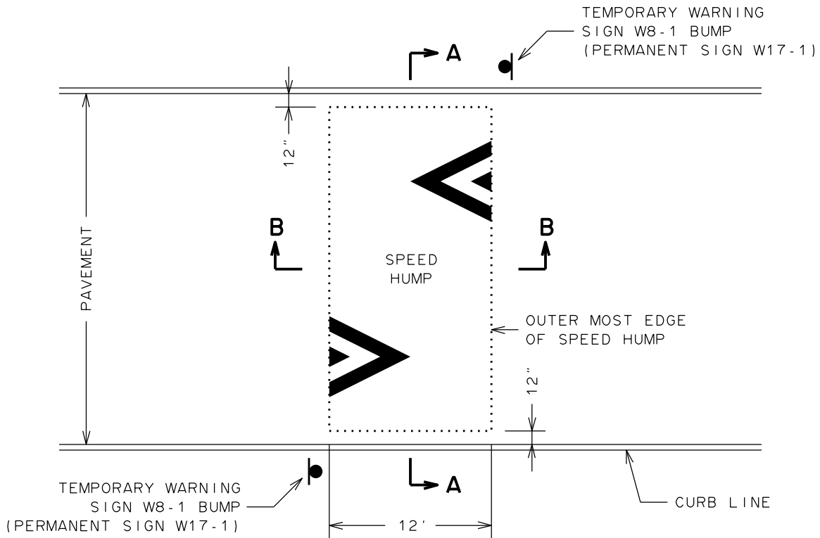
PLAN
