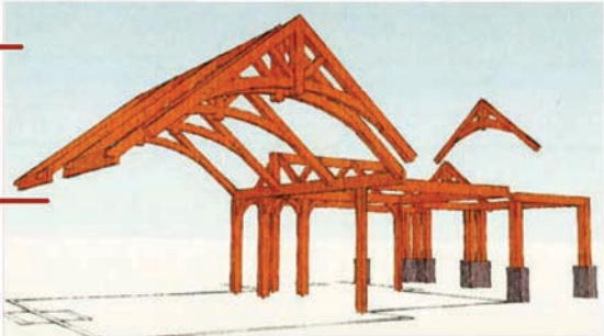
HEAVY TIMBER FRAME
