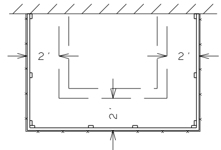
PLAN WITHOUT WALKWAY
