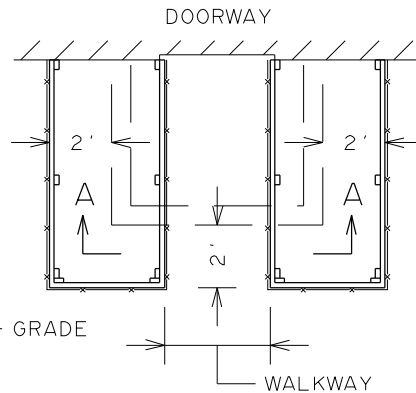
PLAN WITH WALKWAY
