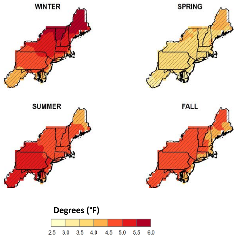
Figure 6. Increase in Seasonal Temperatures by Mid-Century
