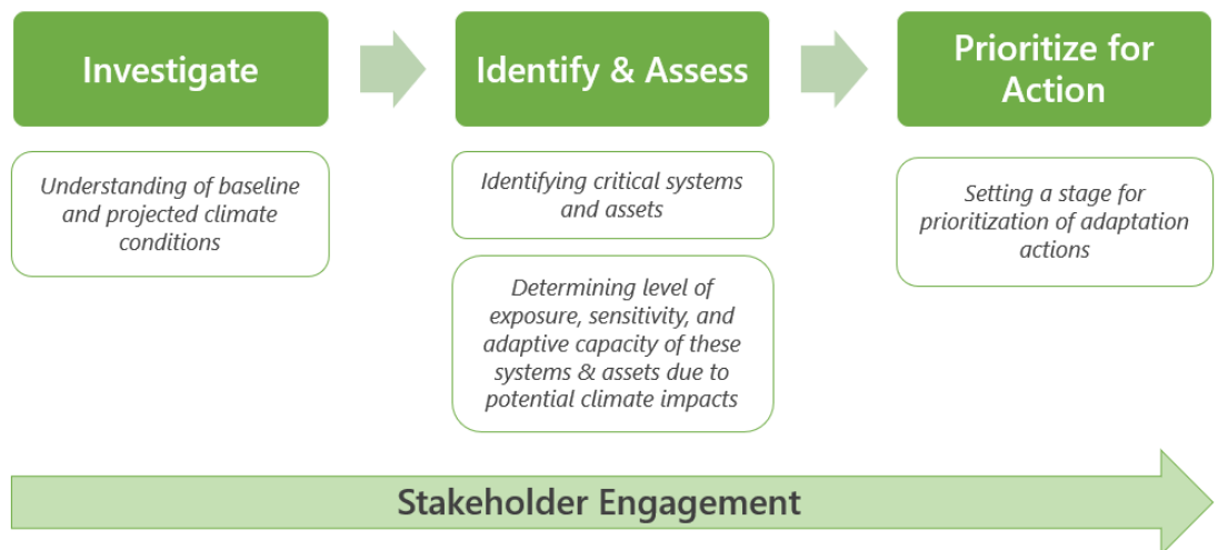
Figure 3. Climate Vulnerability Assessment Approach
