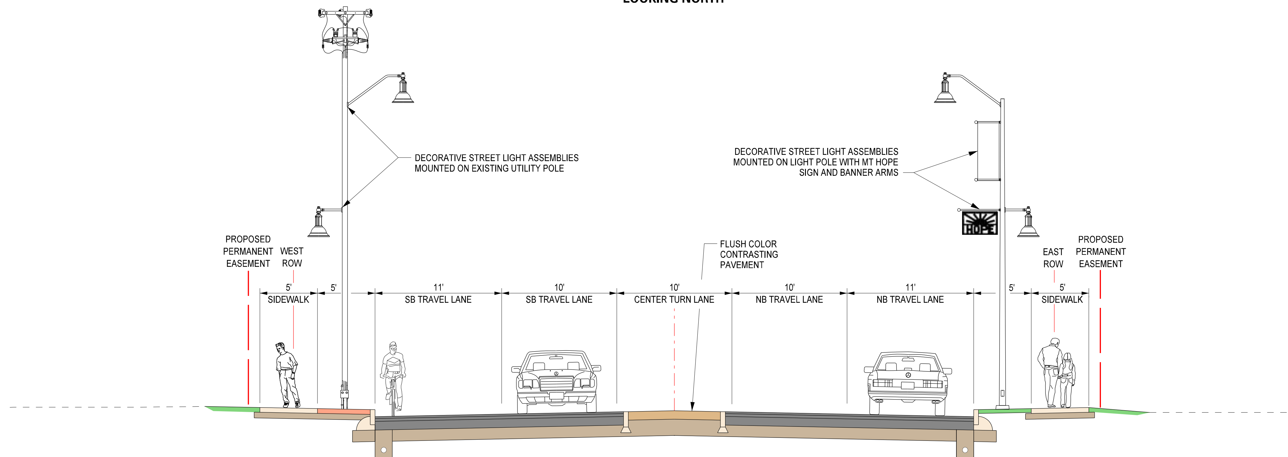
TYPICAL SECTION - EXISTING MOUNT HOPE AVENUE LOOKING NORTH
