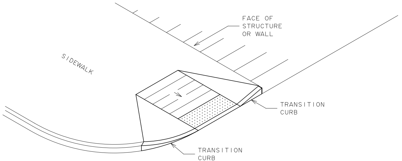
ACCESS RAMP TYPE J
