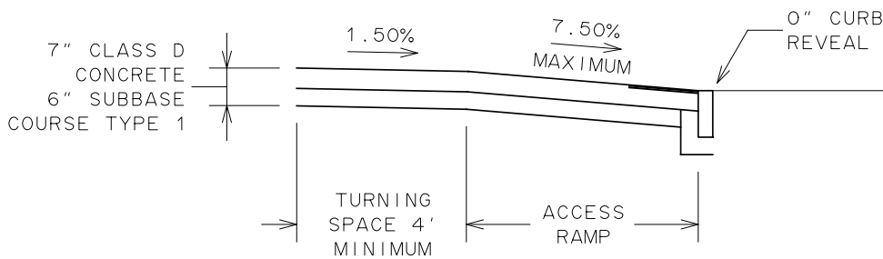
SECTION
