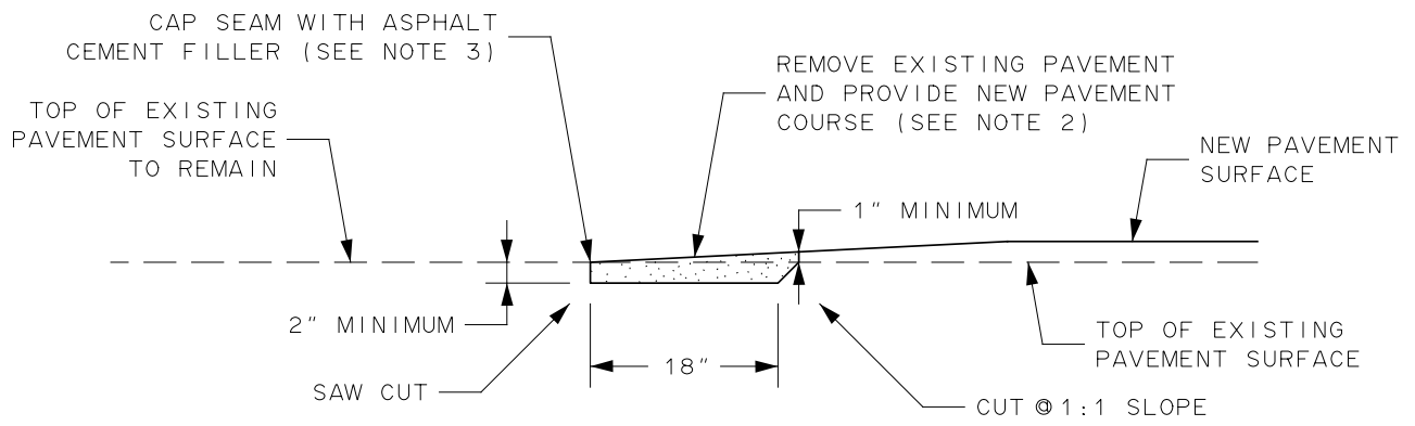
PAVEMENT RESURFACING
