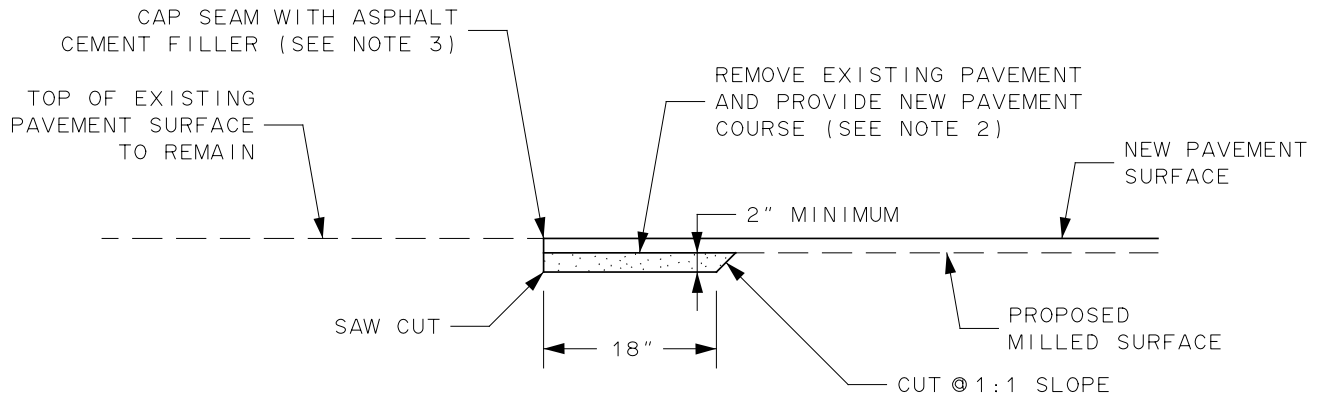
PAVEMENT MILLING
