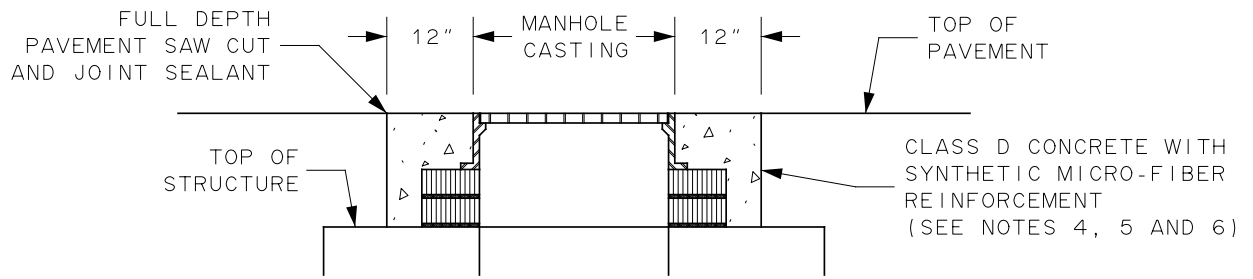
SECTION
