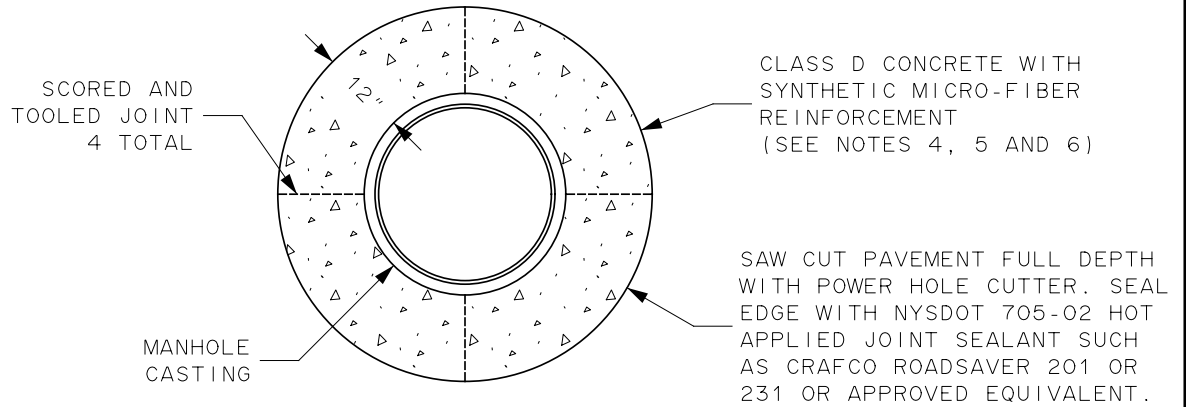
PLAN
