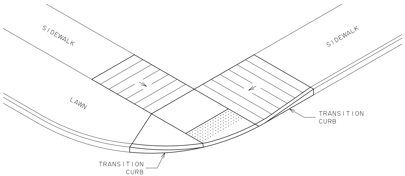
ACCESS RAMP TYPE G
