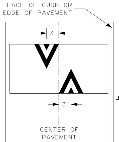
TWO-WAY STREET WIDTH 26' OR LESS
