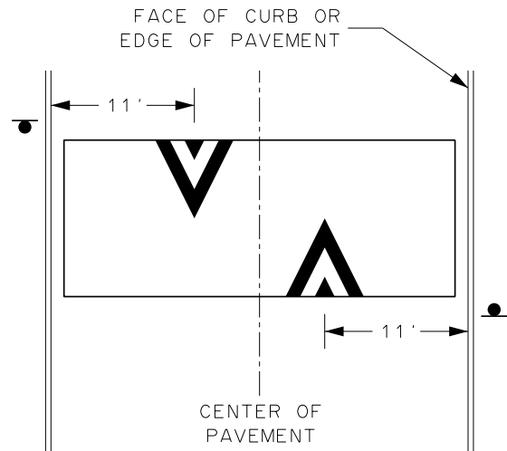
TWO-WAY STREET WIDTH GREATER THAN 26'
