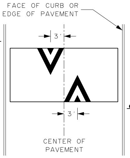
TWO-WAY STREET WIDTH 26' OR LESS
