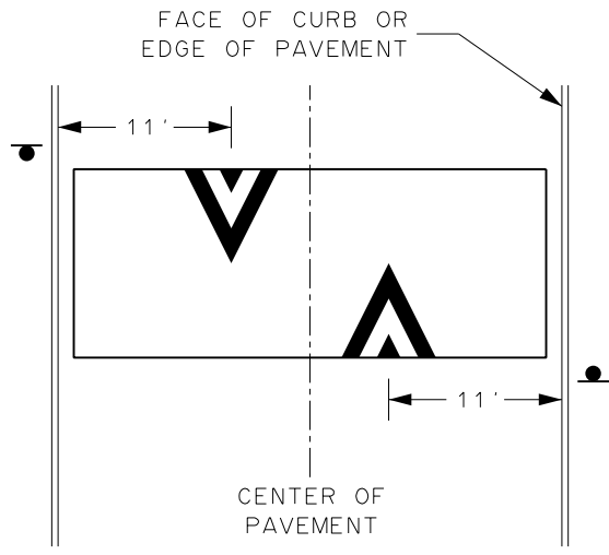
TWO-WAY STREET WIDTH GREATER THAN 26'
